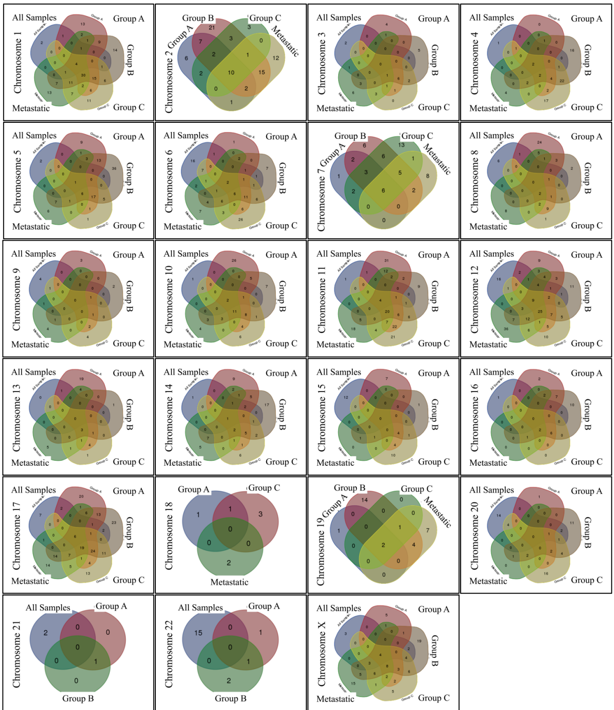
Supplementary Figure 4. Venn diagrams with respect to Chromosomes.
